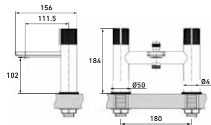
BATH SHOWER MIXER with kit, deck mounted CAS330K1
