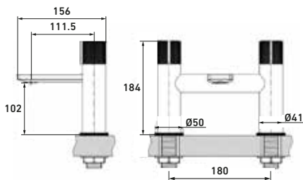
BATH FILLER deck mounted CAS310
